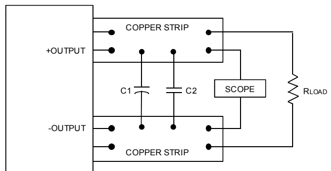
C1=OPEN C2=220µF*3 CERAMIC LOAD 1-2 INCHES (25-51mm) FROM MODULE Figure 5: Measuring Output Ripple and Noise(PARD)
