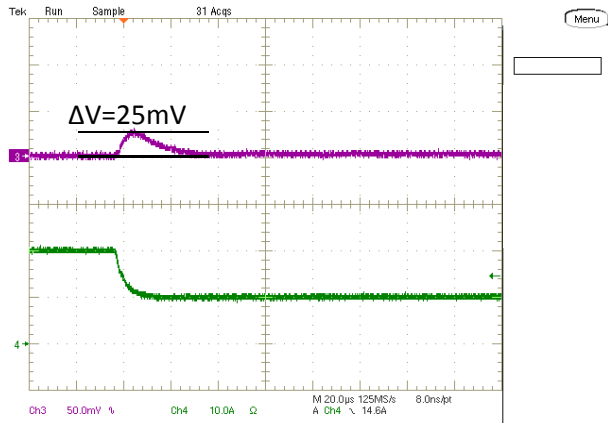
Step Load Transient Response (Vin=12V, Vout=1.0V, Clod=660uF, Iout=20A to 10A, 2.5A/us) Trace 3=Vout, 50 mV/div, Trace 4=Iout, 10A/div.
