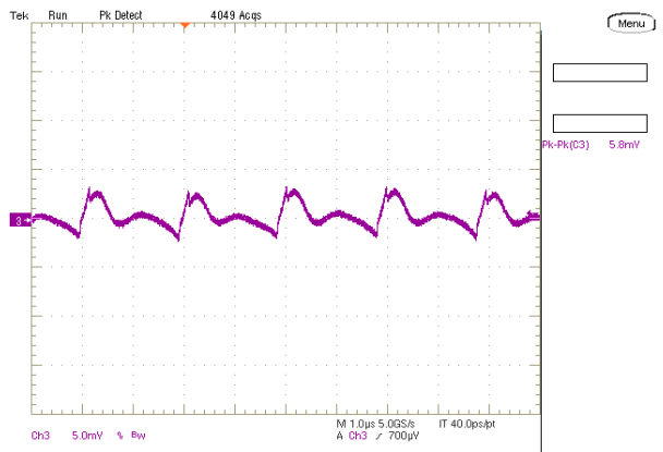
Output Ripple and Noise (Vin=12V, Vout=1.0V, Iout=20A, Clod=660uF, ScopeBW=20MHz)
