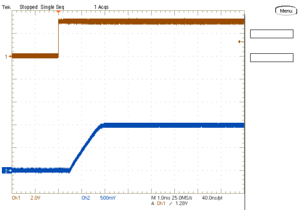
On/Off Enable Delay (Vin=12V, Vout=1.0V, Iout=20A, Clod=660uF) Trace1=Enable, Trace2=Vout
