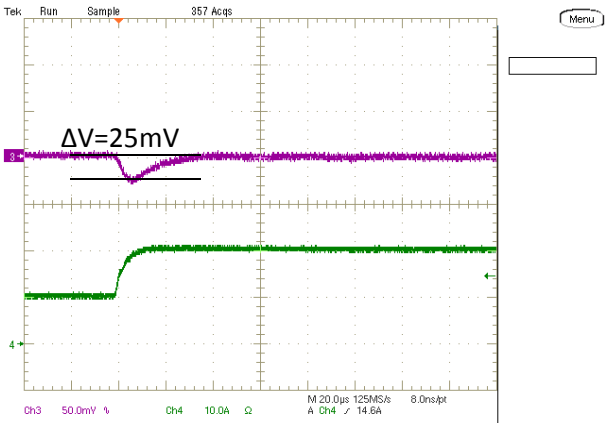
Step Load Transient Response (Vin=12V, Vout=1.0V, Clod=660uF, Iout=10A to 20A, 2.5A/us) Trace 3=Vout, 50 mV/div, Trace 4=Iout, 10A/div.
